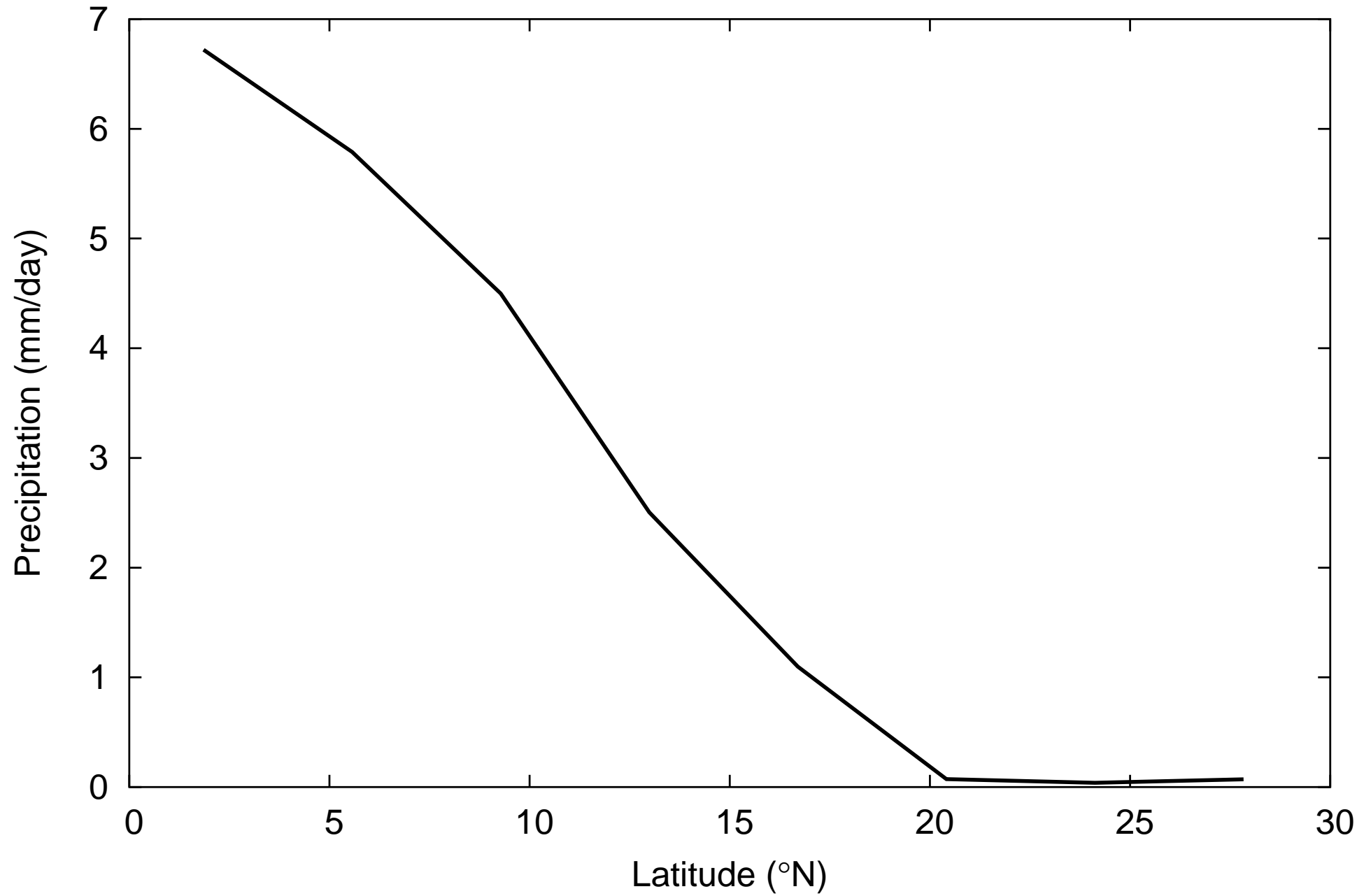
UToronto Zonally Averaged Africa Precipitation (6K OA)
