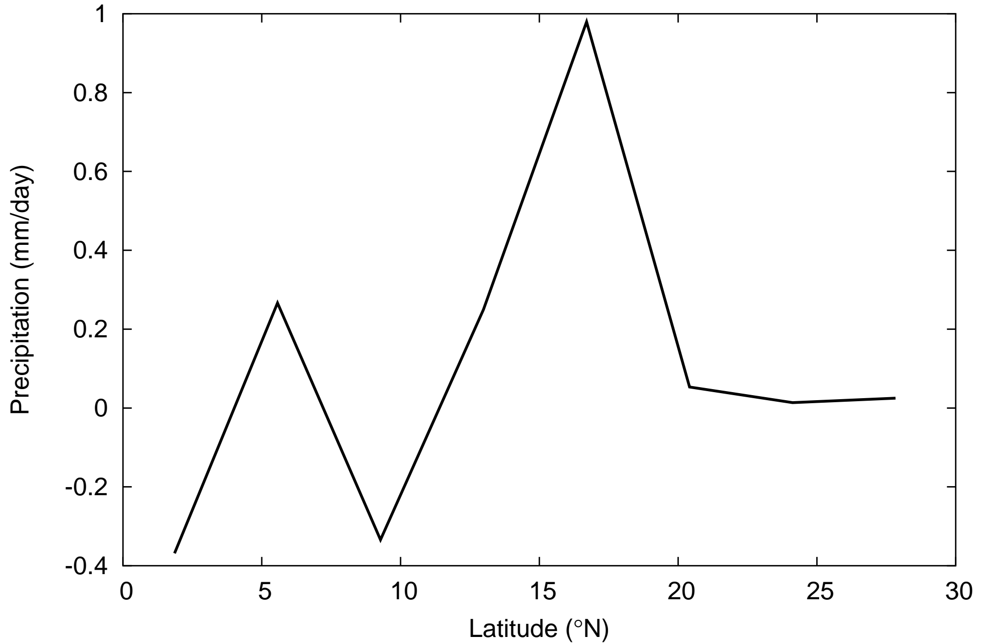
UToronto Zonally Averaged Africa Precipitation (6K OA - 0K OA)
