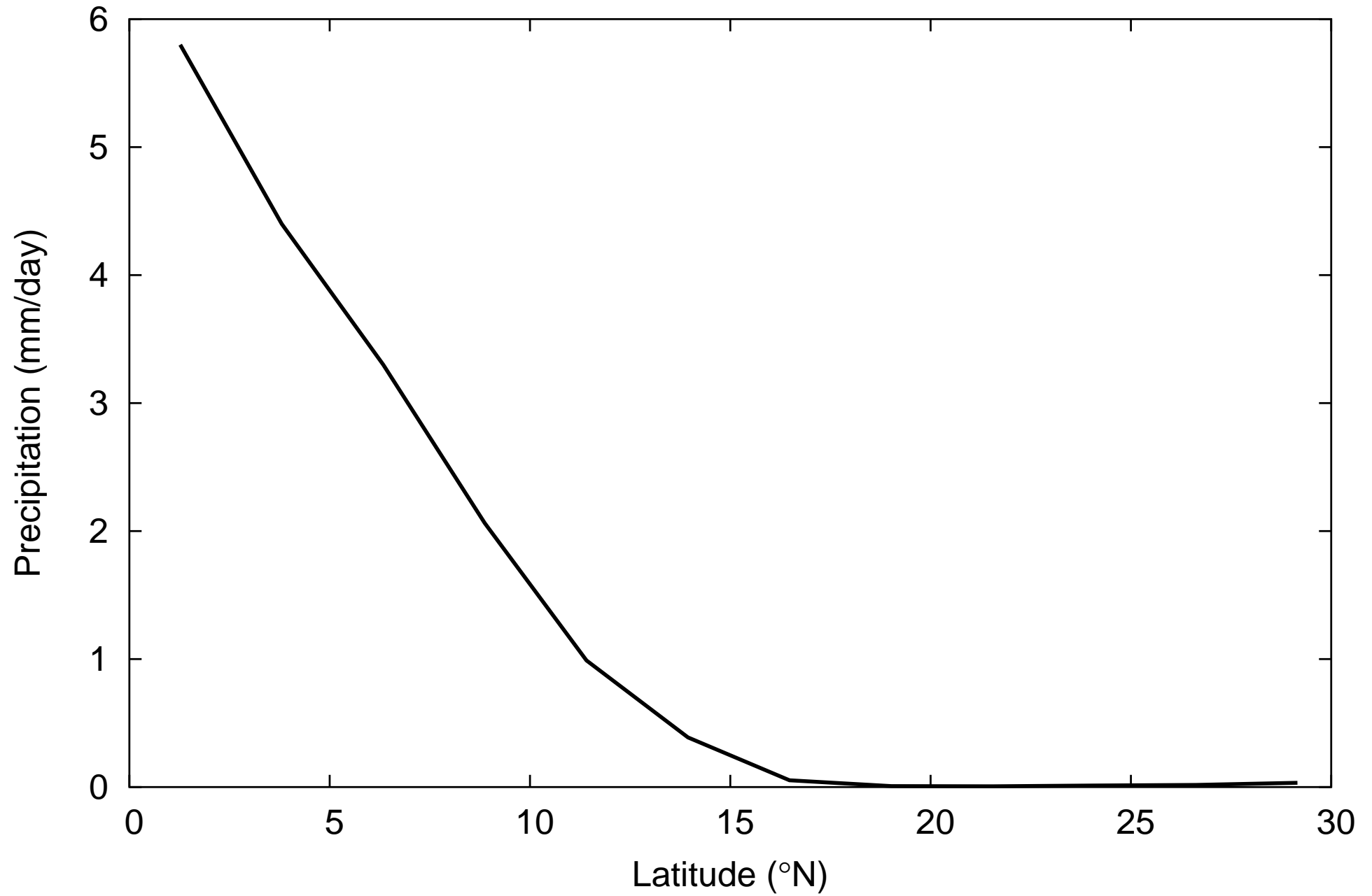
IPSL-CM4-V1-MR Zonally Averaged Africa Precipitation (6K OA)
