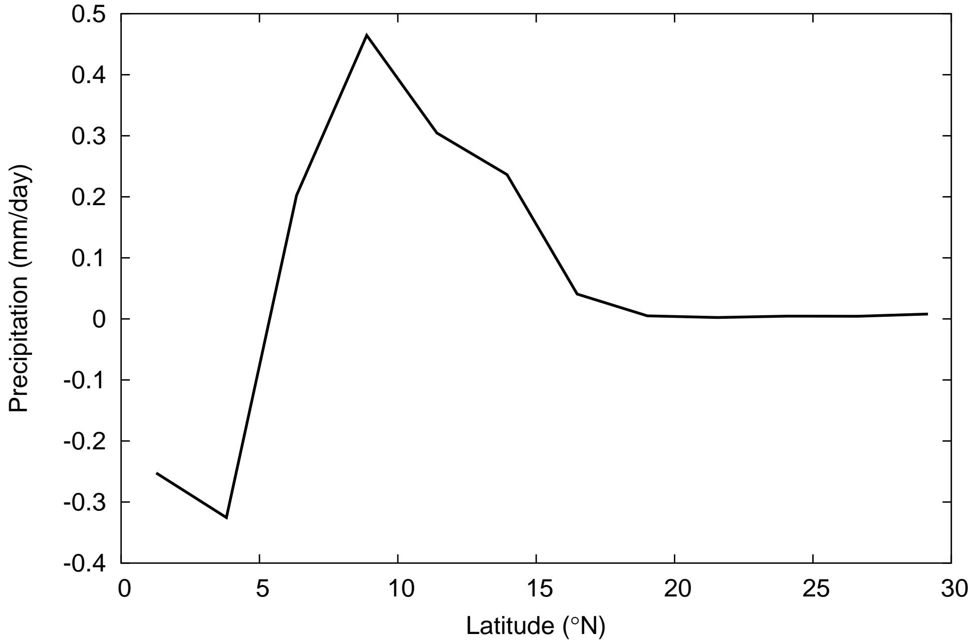
IPSL-CM4-V1-MR Zonally Averaged Africa Precipitation (6K OA - 0K OA)
