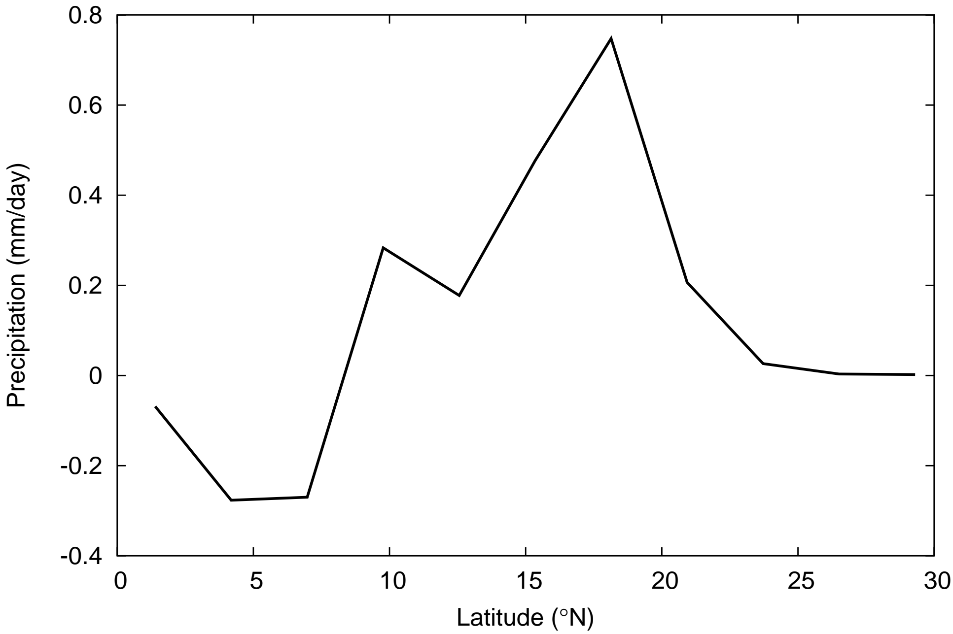
CCSM Zonally Averaged Africa Precipitation (6K OA - 0K OA)
