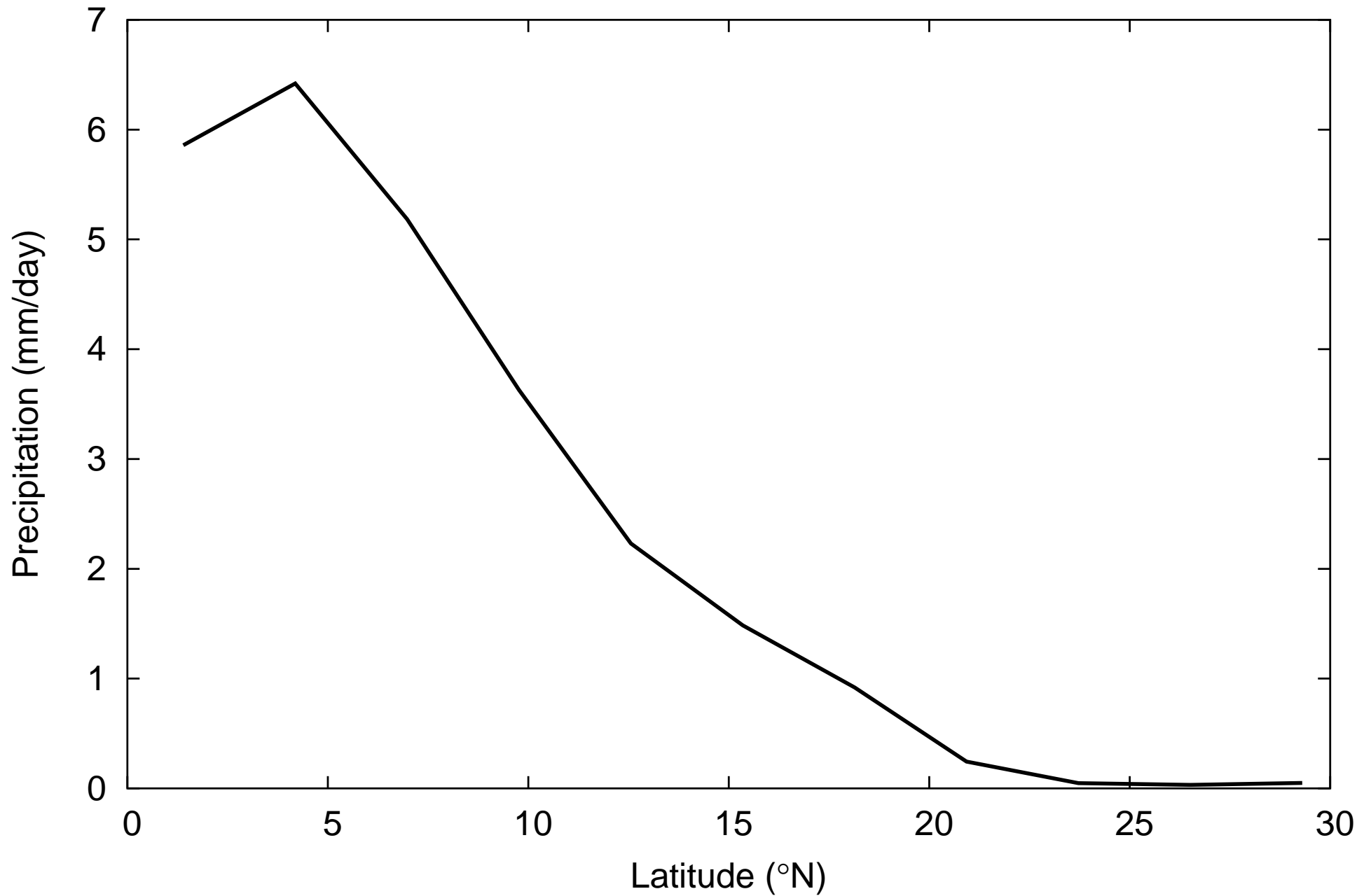
CCSM Zonally Averaged Africa Precipitation (6K OA)
